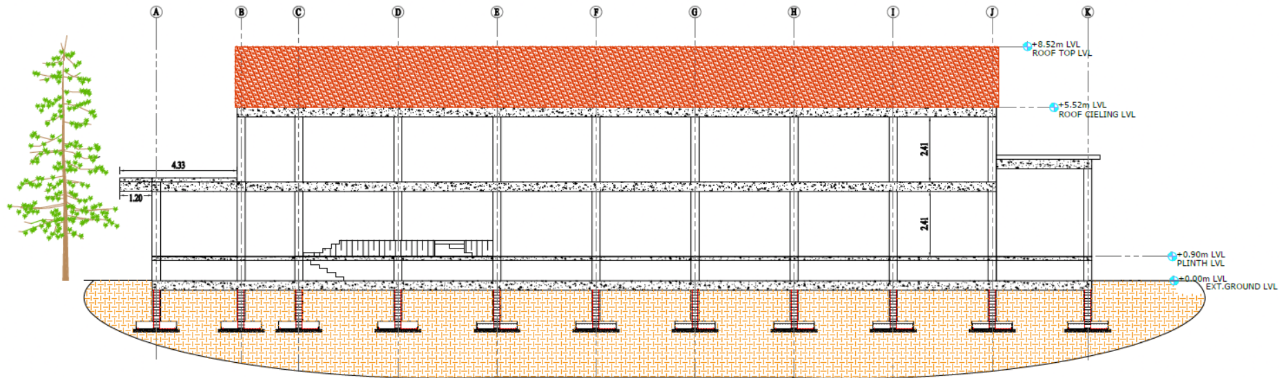
SECTION X-X
