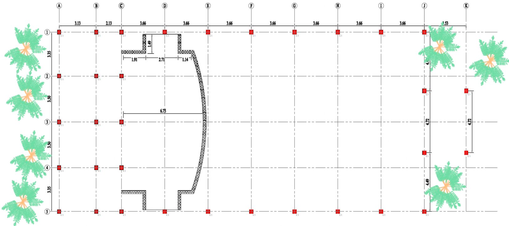
COLUMN LAYOUT WITH BRICK WORK LAYOUT FOR STAGE
