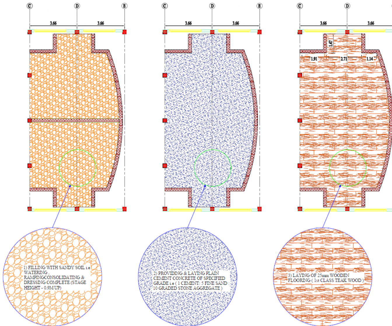
SPECIFICATION OF STAGE
