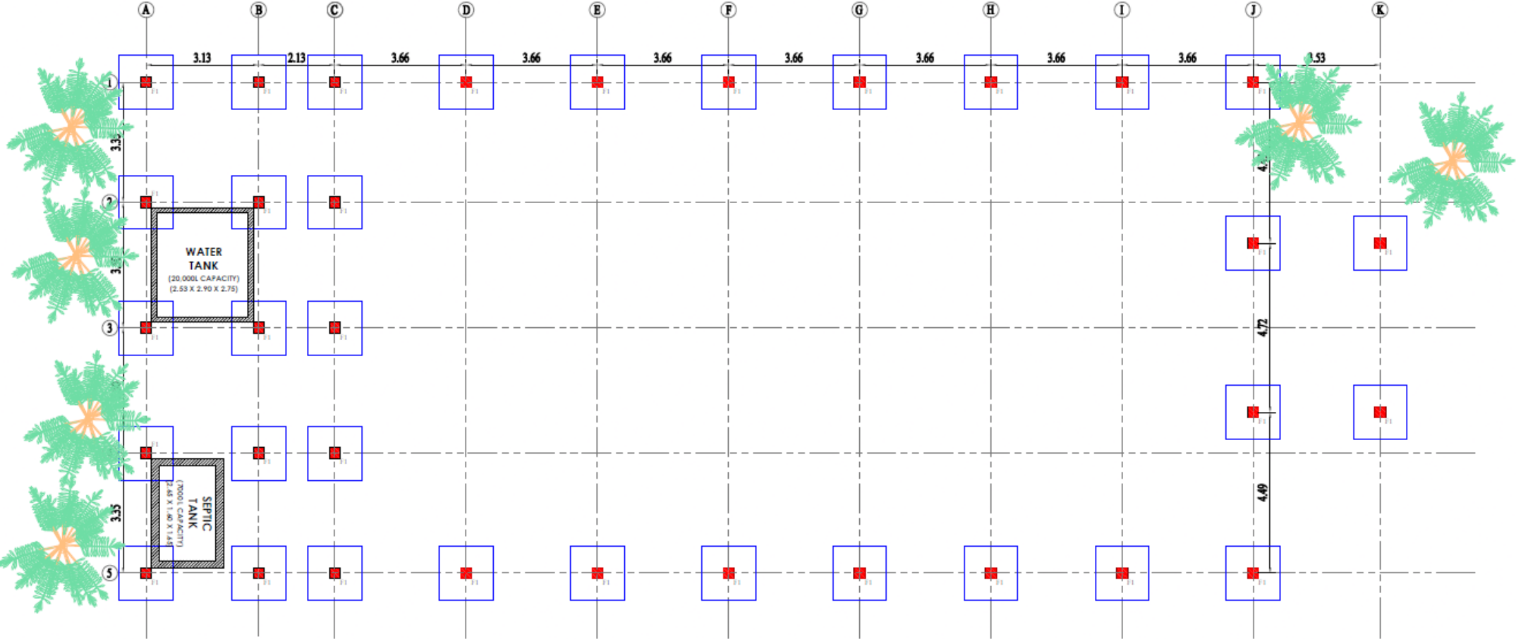
FOOTING LAYOUT, SEPTIC AND WATER TANK PLAN
