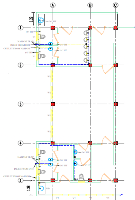
PLUMBING PLAN LAYOUT
