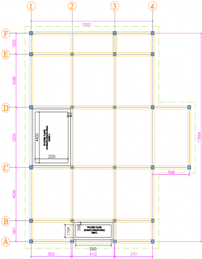
SEPTIC & WATER TANK PLAN
