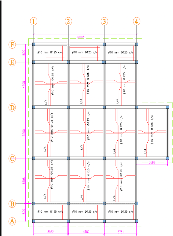
SLAB PLAN & DETAILS
